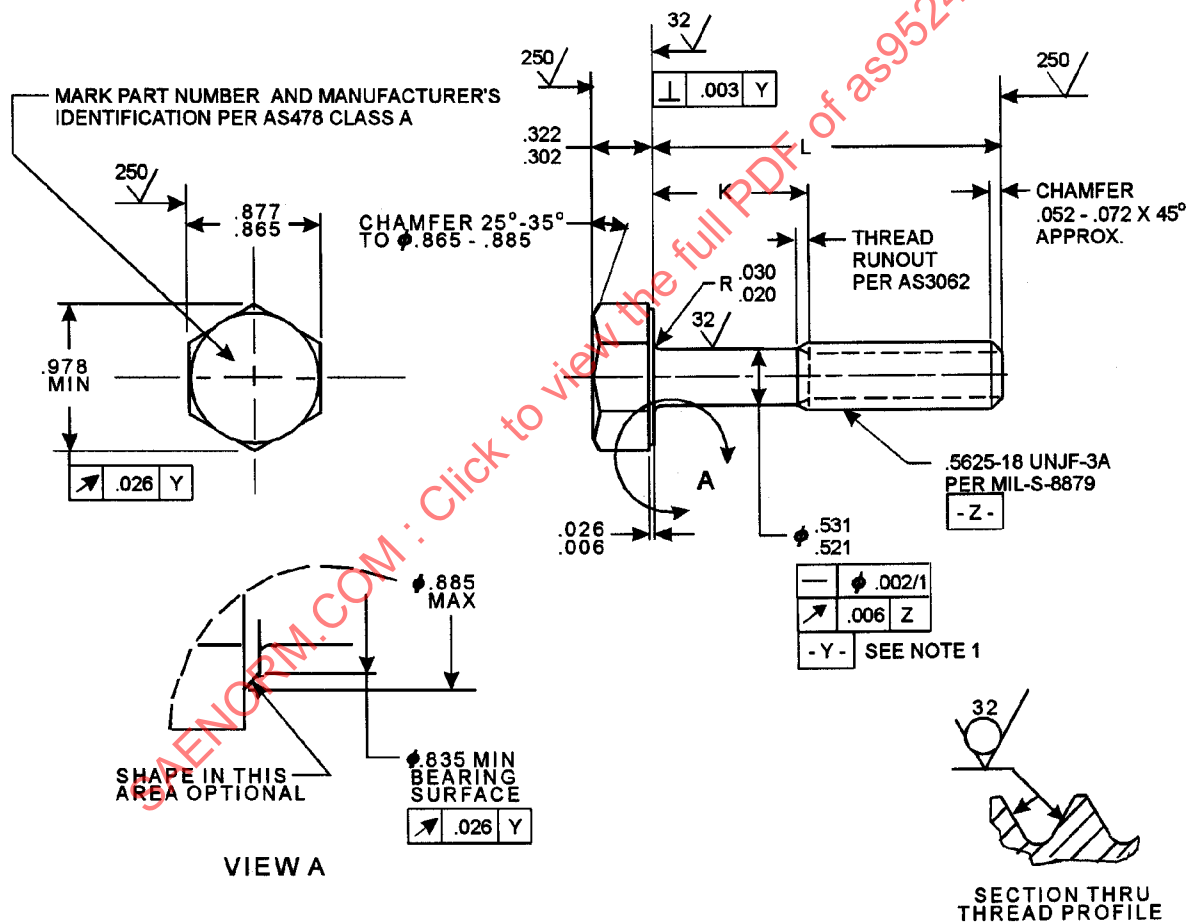
FIGURE 1 - BOLT
