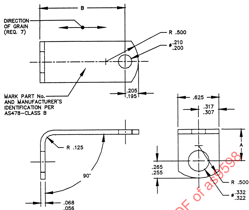
FIGURE 1 - ANGLE BRACKET
