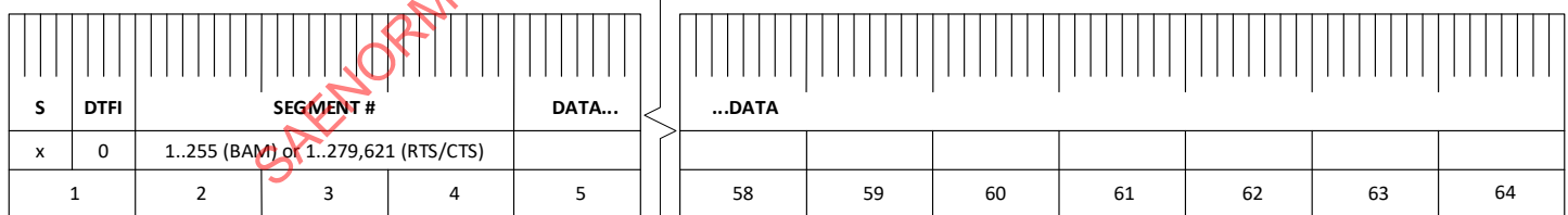
Figure 35 - FD Transport protocol - data transfer message
