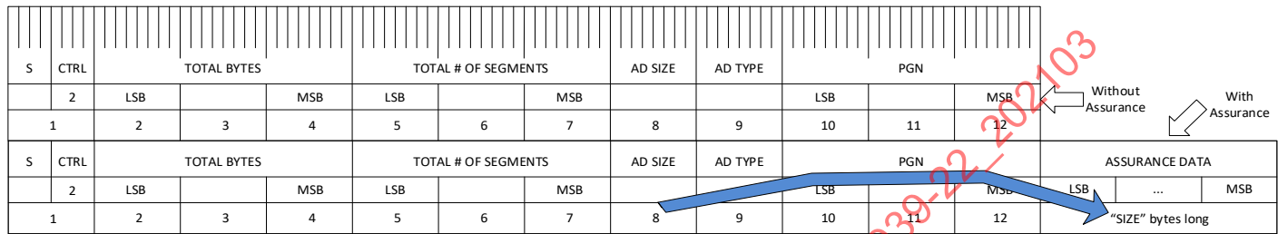
Figure 30 - Data Format of EOMS message
