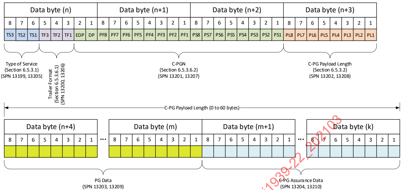
Figure 18B - C-PG Bit Placement Model for TOS=1 and TOS=2
