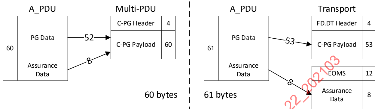
Figure 25 - A_PDU data size
