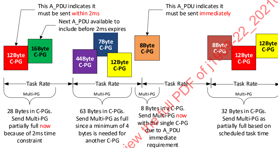
Figure 22 - Transmit control example
