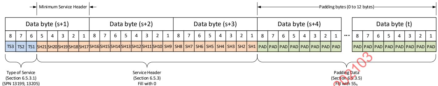
Figure 19B - C-PG Bit Placement Model for TOS=0 (Padding Service)
