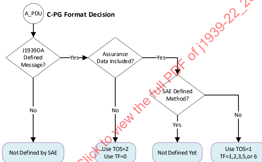
Figure 21 - TOS and TF selection guide
