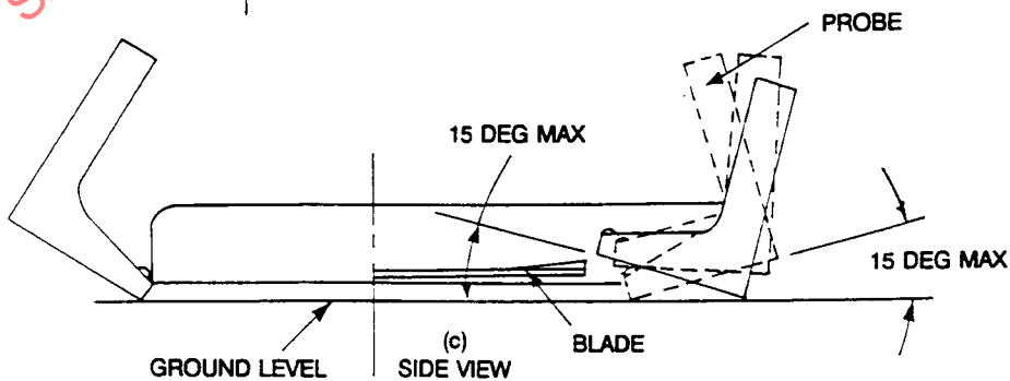
FIGURE 6—FOOT PROBE
