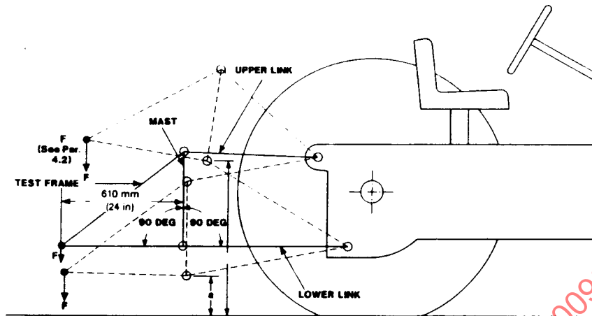
FIGURE 2—TEST FRAME
