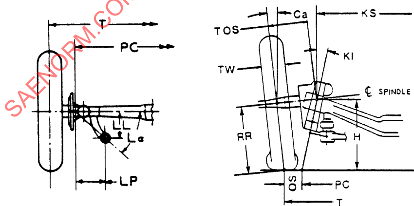
FIGURE 2—DIAGRAM ILLUSTRATING FACTORS OF FRONT AXLE CONFIGURATION
