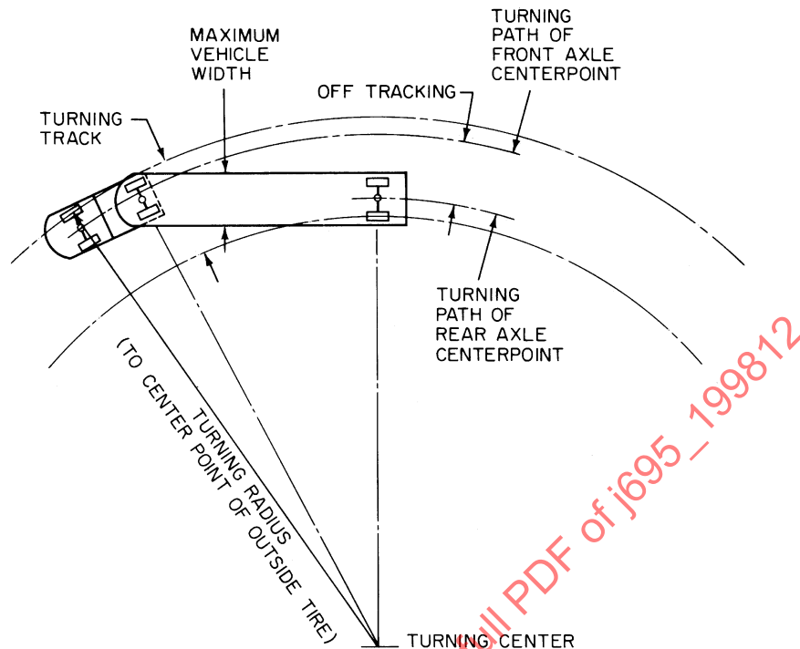
FIGURE 6—TYPICAL OFF TRACKING SITUATION
