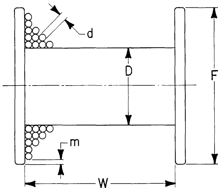
FIGURE 1—DRUM DIMENSIONS
