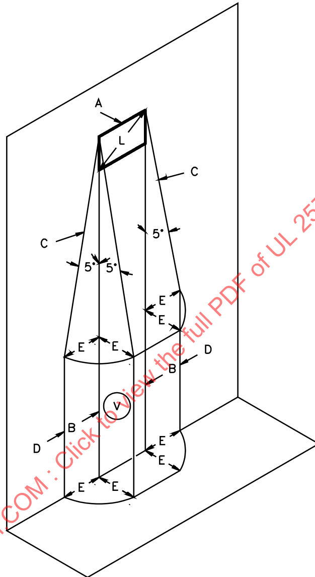
Figure 7.3 Example of enclosure side opening
