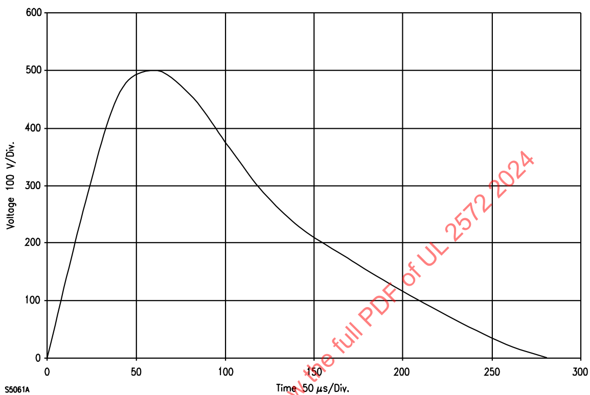
Figure 61.3 Signal line transients – 500V curve
