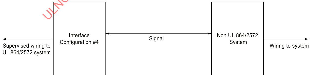
Figure 38.3 TC 4 Isolation Interface
