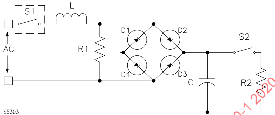
Figure D.1 Typical test circuit diagram
